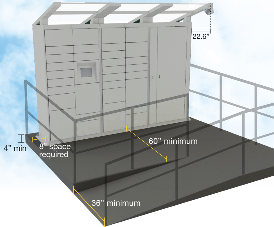
Concrete Pad Option 2: Above Grade
