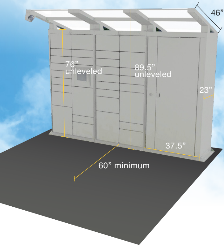
Concrete Pad Option 1: Graded
